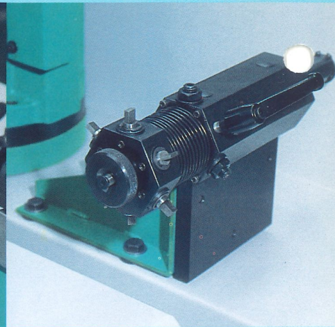
Quick adjusting multi-stylus arrangement (Visage Plus).
