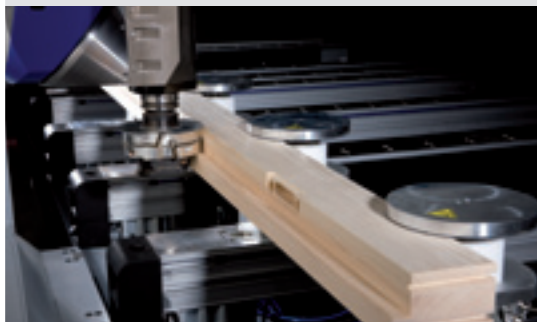
Profiling of frame components
