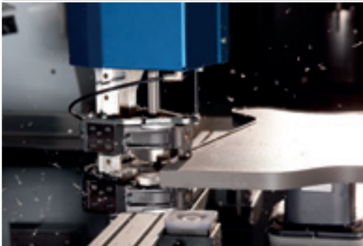
Perfect edge finish with traced combination flush trimming / scraping unit
