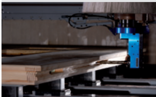
Lock case trimming on front doors
