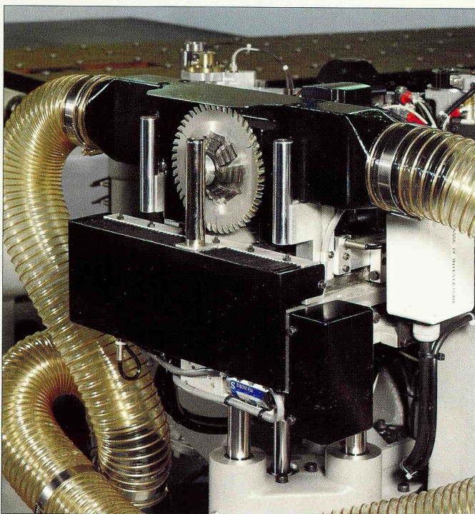
End-trimming unit and rounding unit. Kapp- und Fasaggregat.
