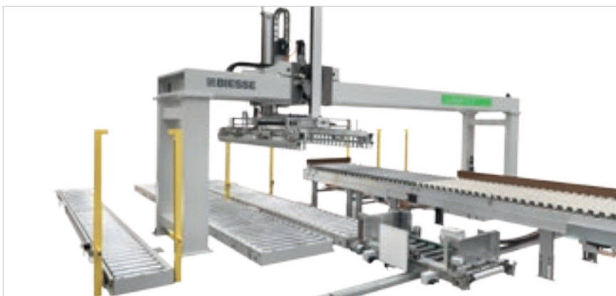
Lifter Bridge unloader for cutting cells.
