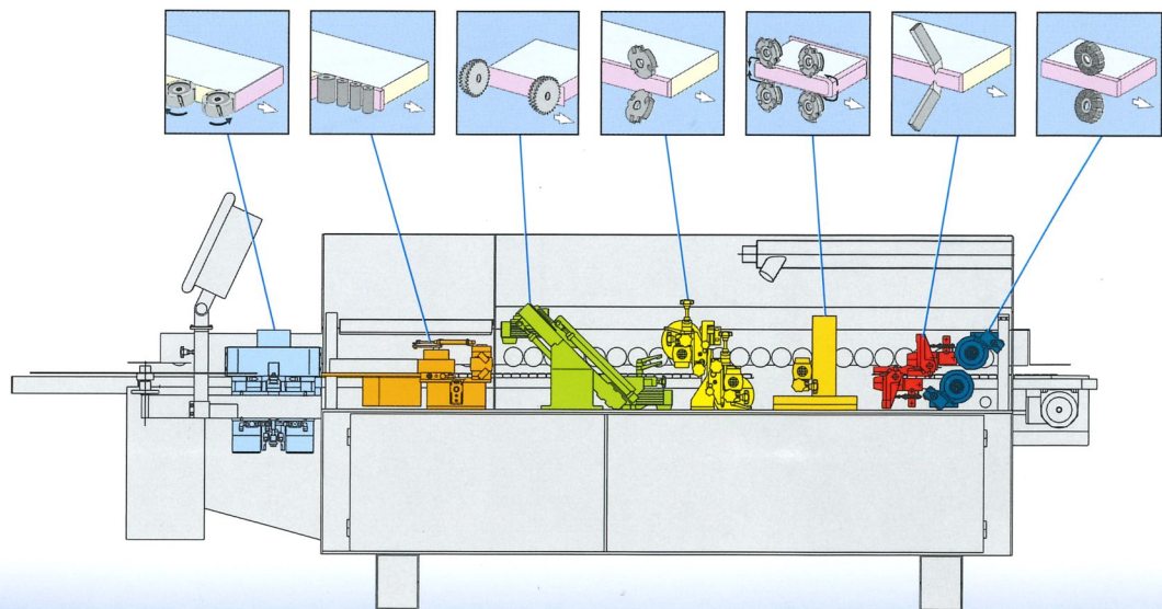
Optimat KDF 350 C
