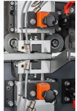
Surface scraper with dual-tracing
