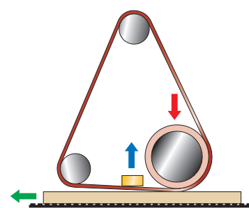
Calibrating / sanding with roller
