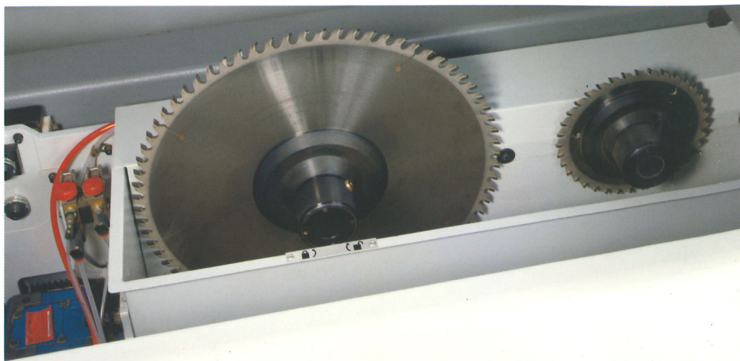
Carro sierra con Quick Change System Carro porta serras com Quick Change System
