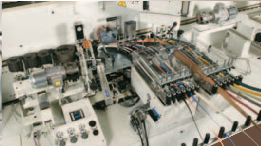
Gluing unit
