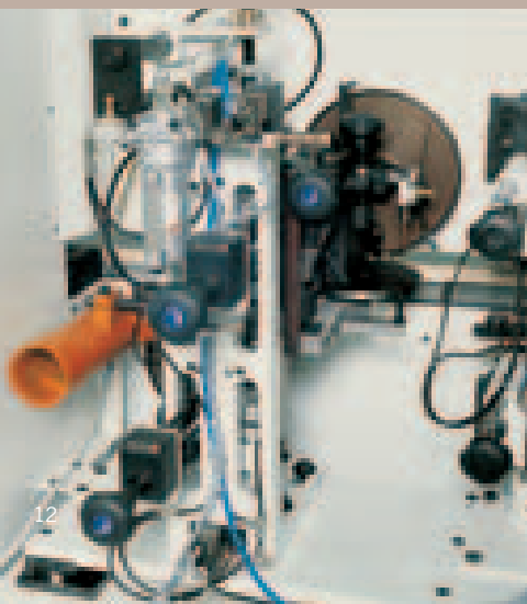
Edgescraping unit
