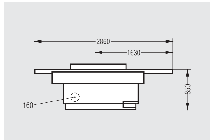
HB = 510 kW = 5,5
