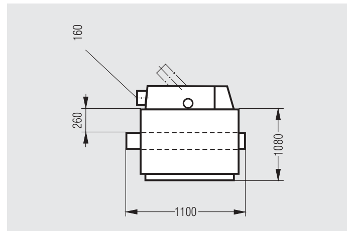
HB = 630 kW = 7,5 + 11
