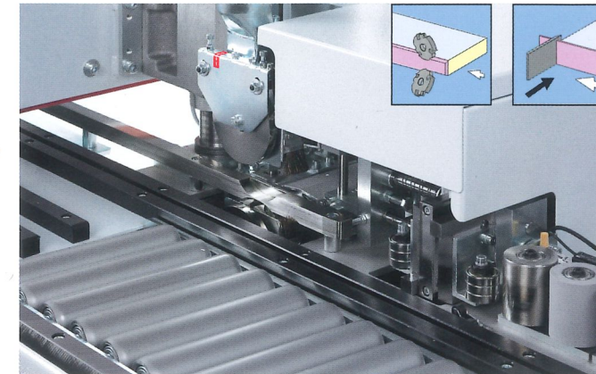
Bündigkappaggregat + Bündigfräsaggregat End trimming and flush trimming Restador a ras + Fresador a ras
