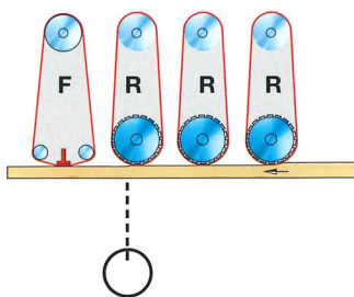
Four head calibrating and finishing sander with three contact rollers and one air cushion pad
