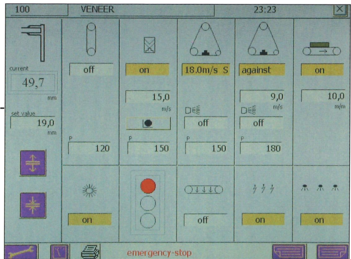
Operator Terminal for complete machine control
