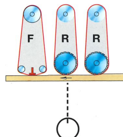
Three head calibrating and finishing sander with two contact rollers and one air cushion pad
