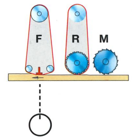
Planer sander with cutter head, contact roller and air cushion pad
