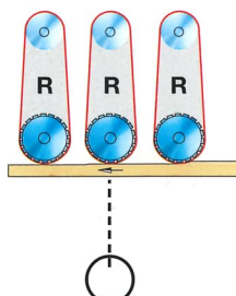
Three head calibrating and finishing sander with three contact rollers
