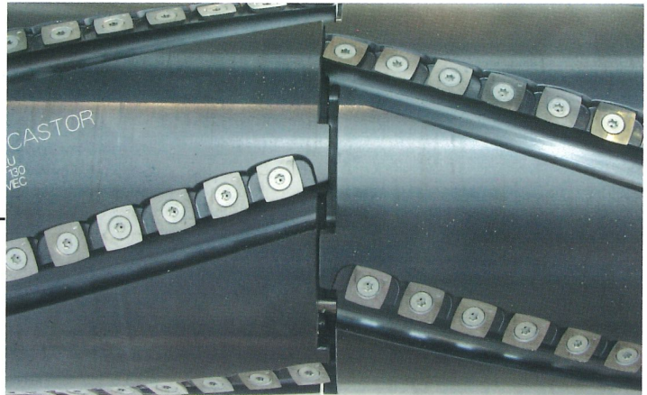
Spiral cutter-block for a perfect cut up to 4 mm / 0.16 inch in one pass
