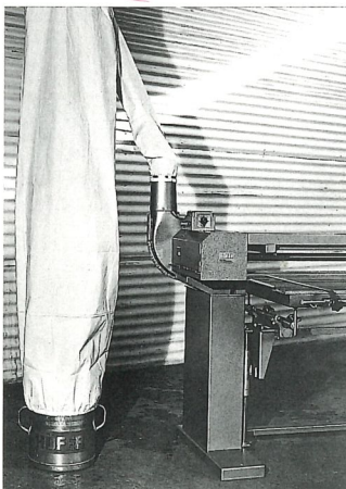
Klein-Staubfilteranlage Dust filter equipment
