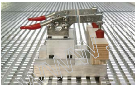
Grooved aluminium matrix table guarantees precise fixture through mechanical clamping elements in any optional location
