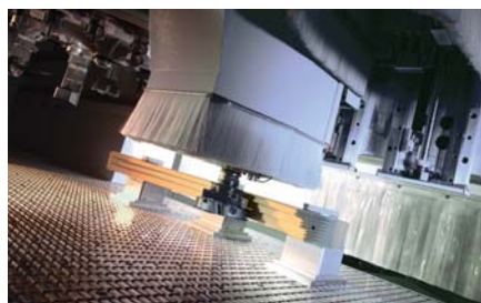
Window production with multi clamp
