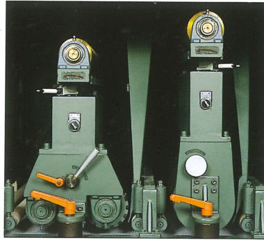
Side view of drum head w/combination head system.
