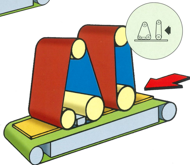
■ ROLLER FOLLOWED BY COMBINATION ROLLER AND PAD (DA type)
