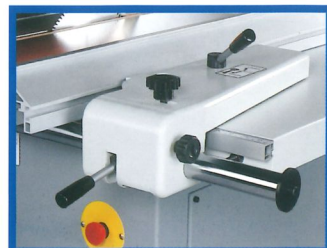
Solid cast iron body and rail to support sturdy cutting, manual fine adjustment with high/low profile.
