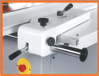
Solid cast iron body and rail to support sturdy cutting, manual fine adjustment with high/low profile.
