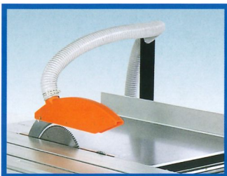
Hose support plate and hose
