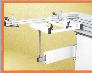
Strong outtrigger and large support roller for loading panel smoothly.
