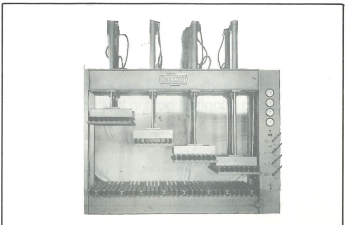
Special FSH Downstroke Press with four separate top tables and rollers in bottom table.
