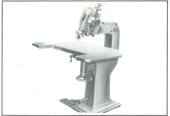
OFC Routing Machine with Canting Head.
