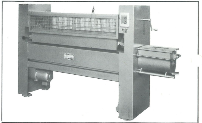
GST Glue Spreading Machine with built on glue mixing unit.
