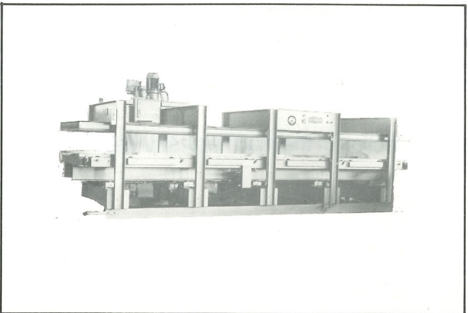
Special EHE type End Loading Upstroke Press with powered conveyor.
