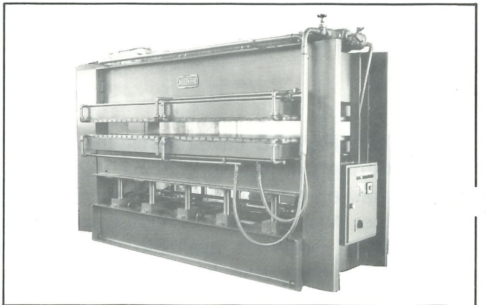
Special HSP type Upstroke Press, oil heated with two solid steel platens.
