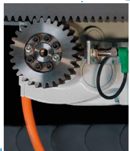
Saw carriage with high precision drive via a gear and rack system.
