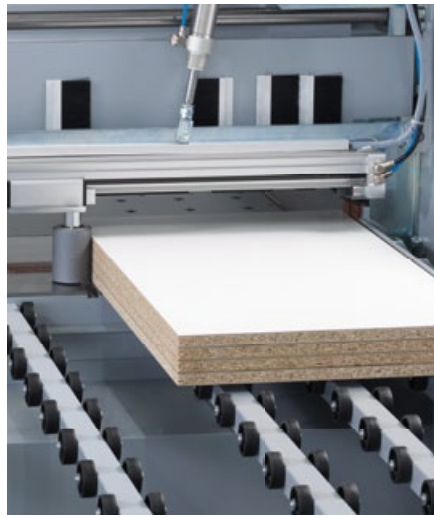
Angle pressing device for a gentle and precise alignment of the panels.
