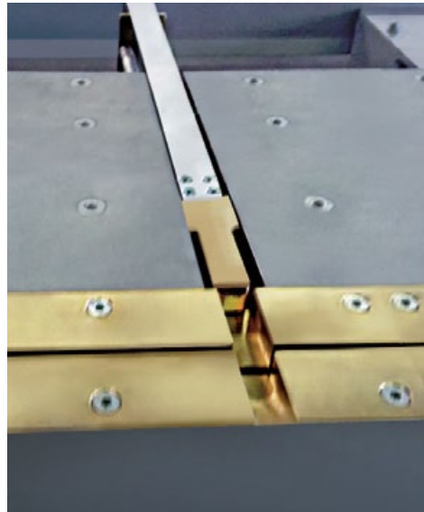
Cutting gap closer for narrow trimming cuts.
