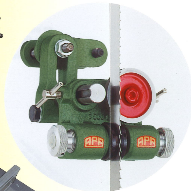
mechanic vertical setting by handwheel with blocking pinion
