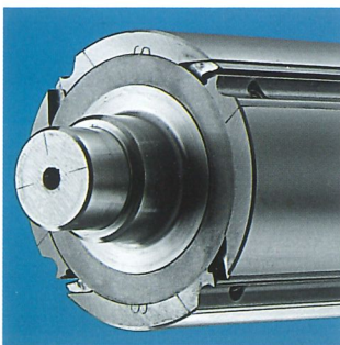
Fliehkraft-Wendemessersystem "Tersa"
