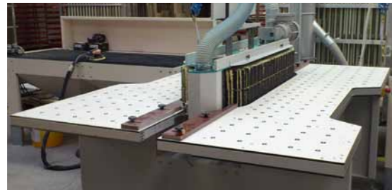
Twin Duplex with two sanding areas placed in a sanding island
